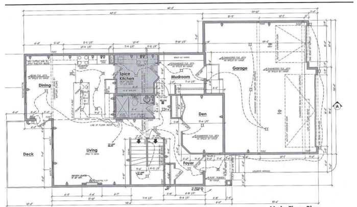
Main Floor Plan 1196 sq ft 9\"/>
