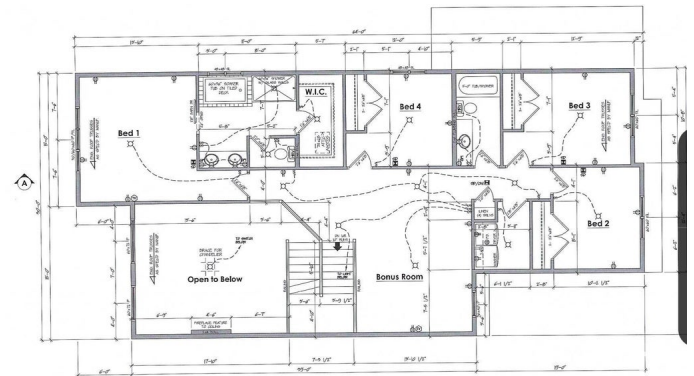
Second Floor Plan 1350 sq ft 9\"/>
